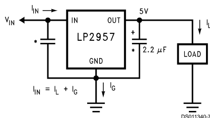
FIGURE 1. Basic 5V Regulator Circuit
