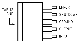
Plastic Surface Mount Package 5-Lead TO-263 (S)
