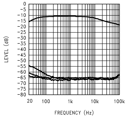
Power Supply Rejection Ratio vs Bypass Capacitor Size V_{DD} = 5V , Input Grounded = 10Ω, Output Load = 8Ω
