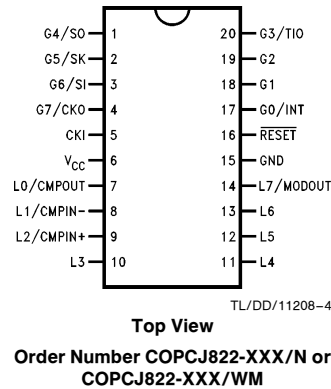
FIGURE 3. Connection Diagrams
