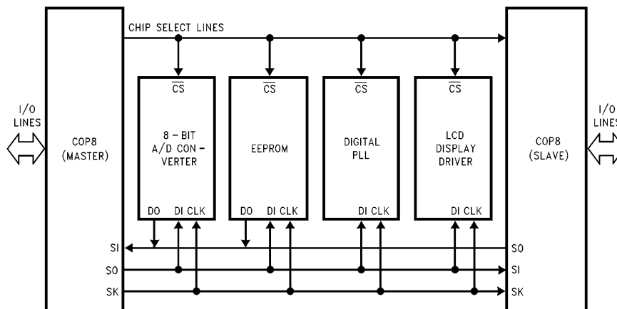
FIGURE 7. MICROWIRE/PLUS Application
