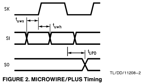
FIGURE 2. MICROWIRE/PLUS Timing
