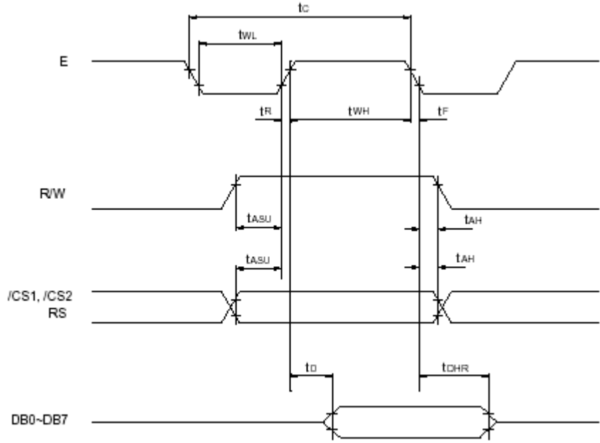
Fig.2 MPU Read Timing
