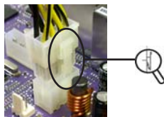
8-pin power cable
