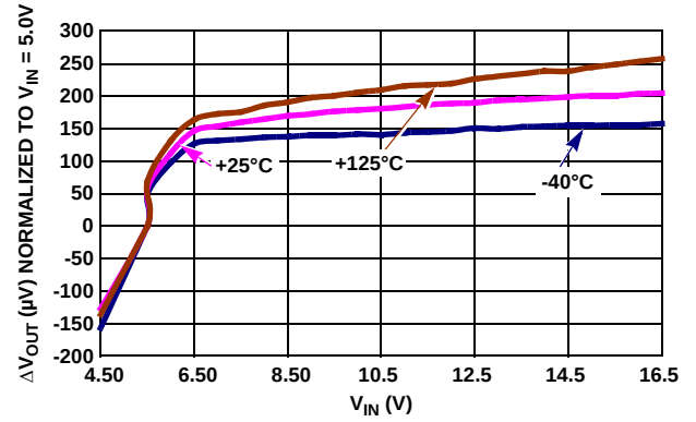
FIGURE 33. LINE REGULATION OVER-TEMPERATURE
