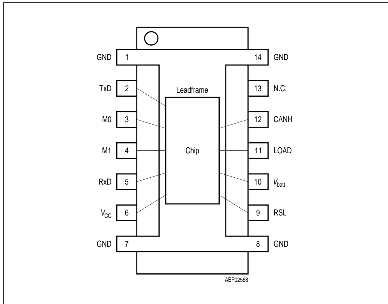
Figure 1 Pin Configuration
