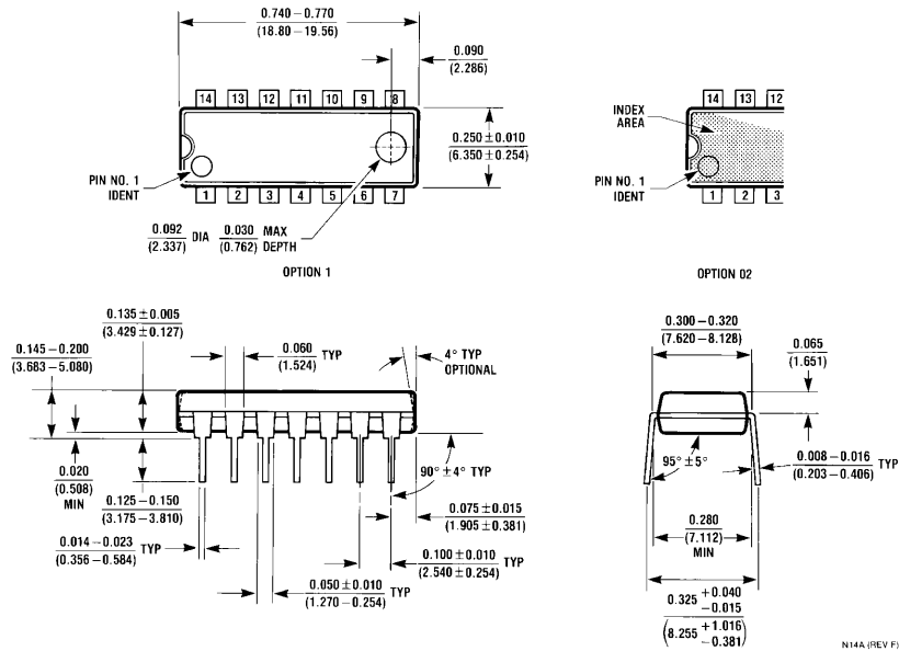
Molded Dual-In-Line Package (N) Order Number ADC08234BIN or ADC08234CIN NS Package Number N14A
