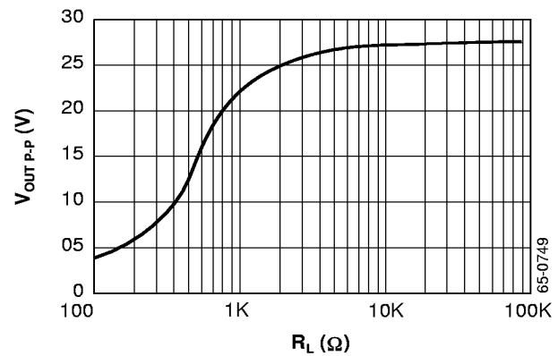
Figure 9. Output Voltage Swing vs. Load Resistance
