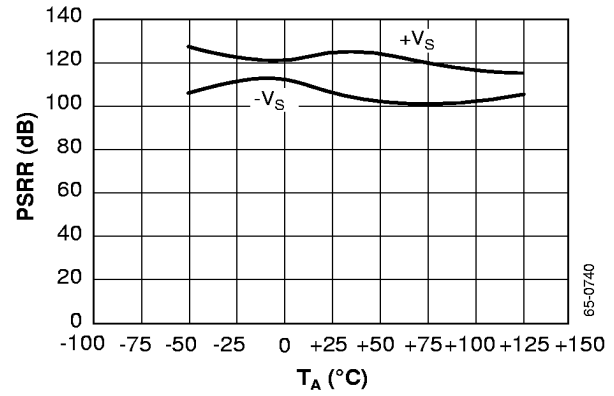
Figure 2. PSRR vs. Temperature
