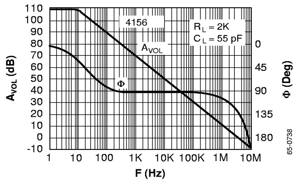
Figure 1. Open Loop Gain, Phase vs. Frequency
