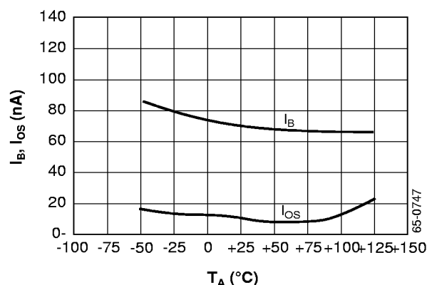
Figure 11. Input Bias, Offset Current vs. Temperature
