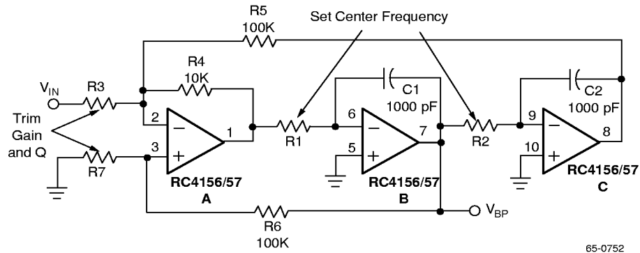
Figure 16. Bandpass Active Filter
