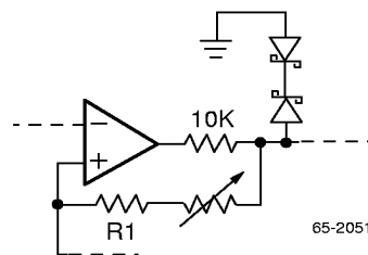
Figure 14. Triangle Generator—Symmetrical Output Option
