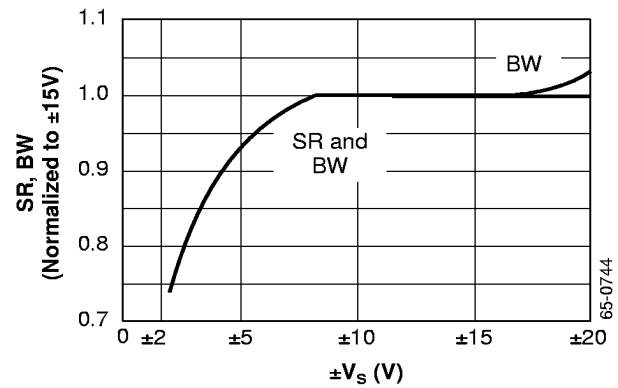
Figure 7. Slew Rate, Bandwidth vs. Supply Voltage
