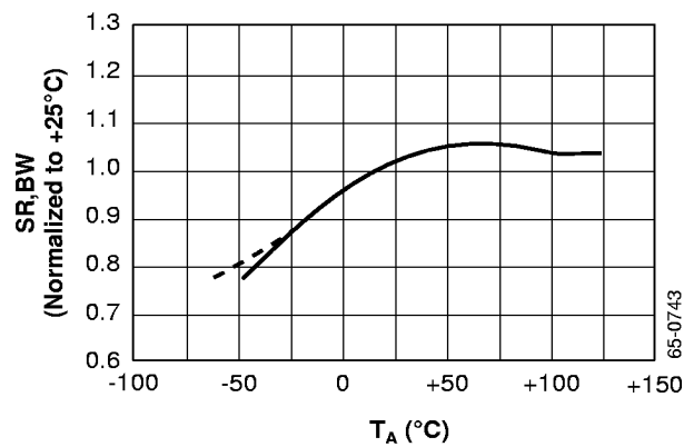
Figure 6. Slew Rate, Bandwidth vs. Temperature
