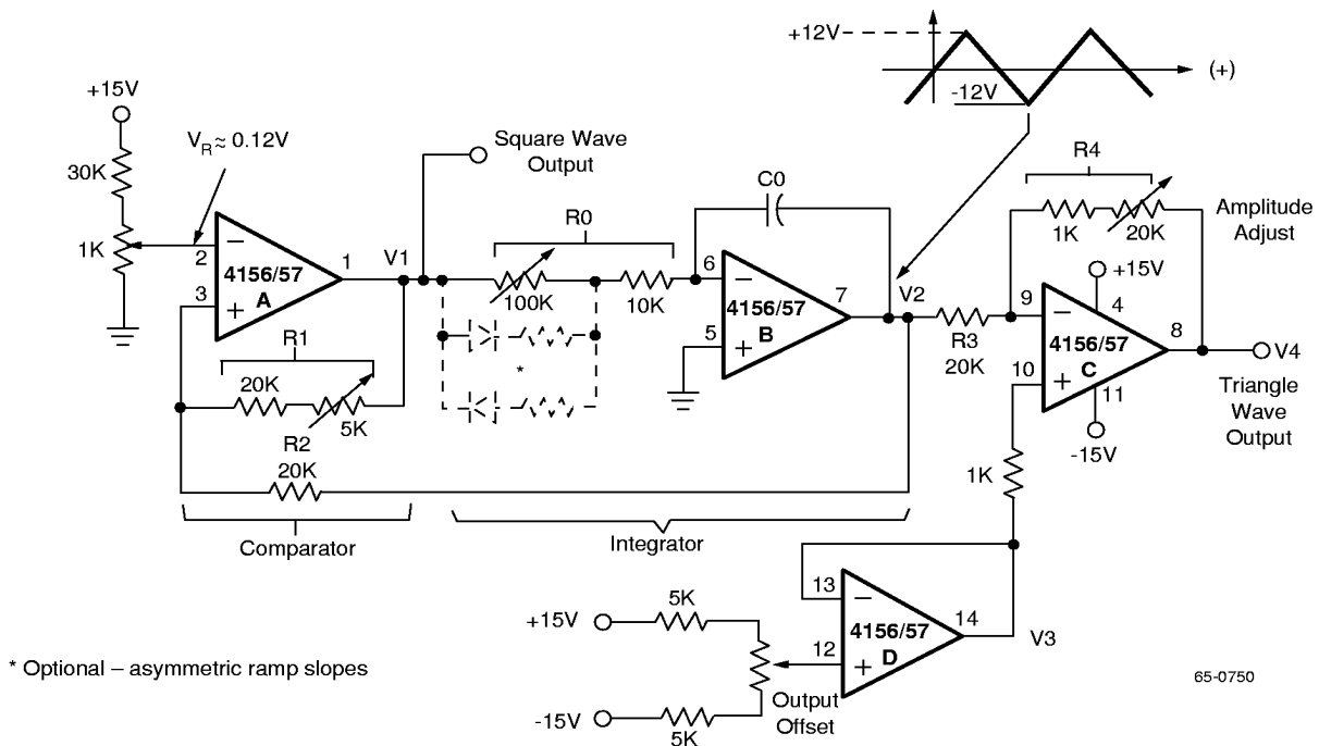
Figure 13. Triangle and Square Wave Generator
