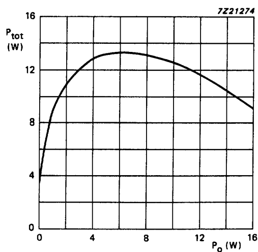
Fig.7 Power dissipation as a function of output power; symmetrical supply; V_P = \pm 16 \text{ V} ; R_L = 8 \Omega ; f = 1 \text{ kHz} .
