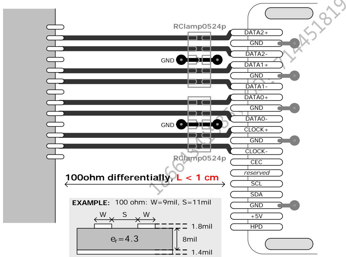
Figure 20. Layout example for high-speed TMDS differential signals
