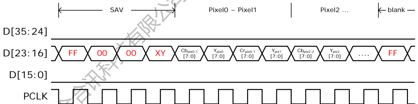
Figure 12. 8-bit CCIR-656
