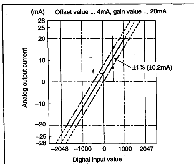
Fig. 2.7 Overall accuracy of current output characteristics
