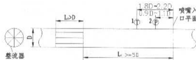
1-温度计; 2-压力计
