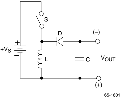
Figure 7. Simple Inverting Regulator
