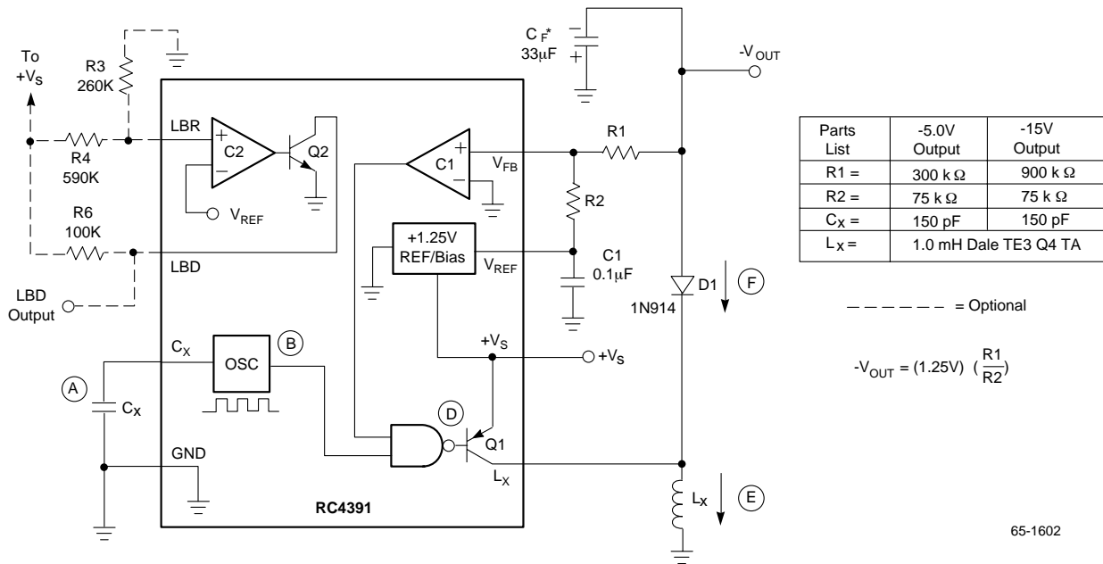
Figure 8. Inverting Regulator – Standard Circuit
