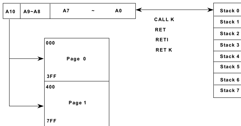
Fig. 4 Program counter organization
