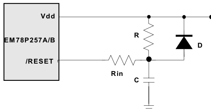
Fig. 18 External Power on Reset Circuit
