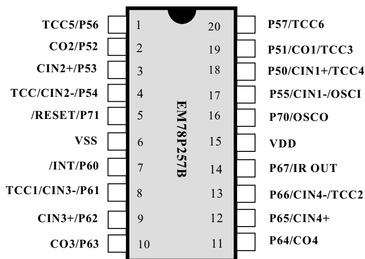
Fig. 2 Pin Assignment - EM78P257B
