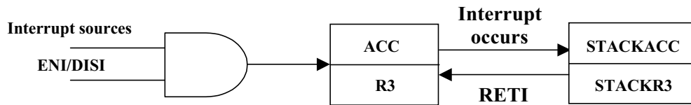
Fig. 13 Interrupt backup diagram
