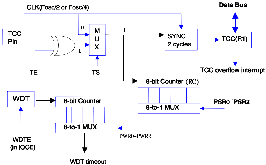
Fig. 6 Block Diagram of TCC and WDT
