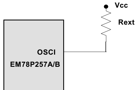
Fig. 26 Circuit for Internal C Oscillator Mode
