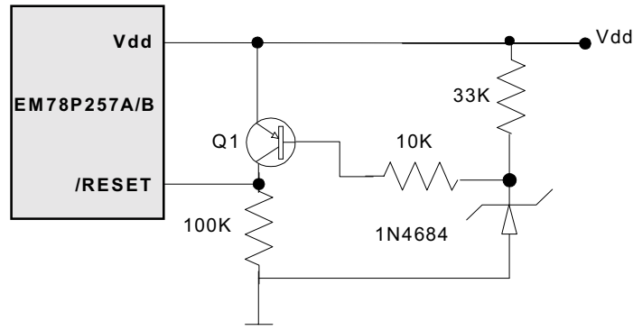
Fig. 19 Circuit 1 for the residue voltage protection
