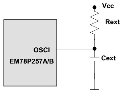
Fig. 25 Circuit for External RC Oscillator Mode
