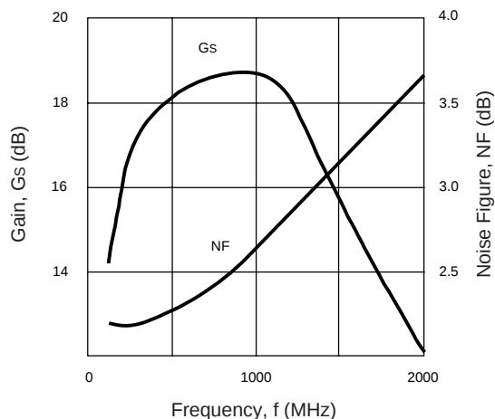
NOISE FIGURE AND GAIN vs. FREQUENCY V_{CC} = 3.0 \text{ V} , I_{CC} = 6 \text{ mA}
