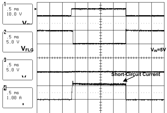
Enabled Into Short (AP1212H)
