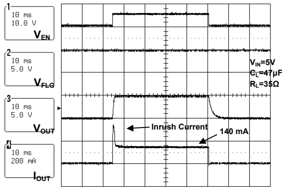
Turn-On/Turn-Off (AP1212H)
