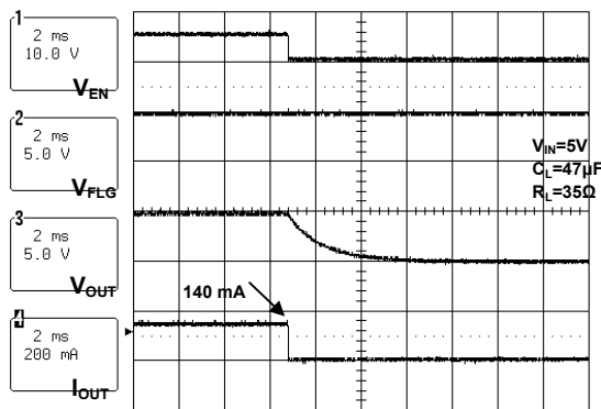
Turn-Off (AP1212H)
