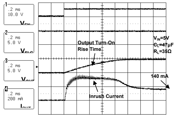
Turn-On (AP1212H)
