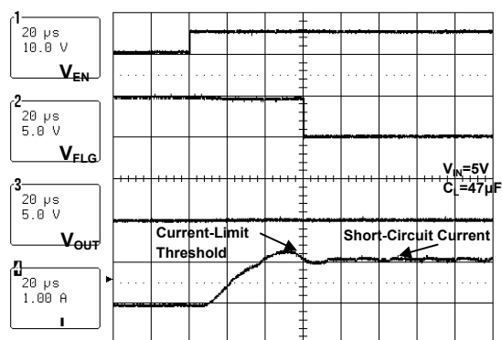
Current-Limit Response (AP1212H)
