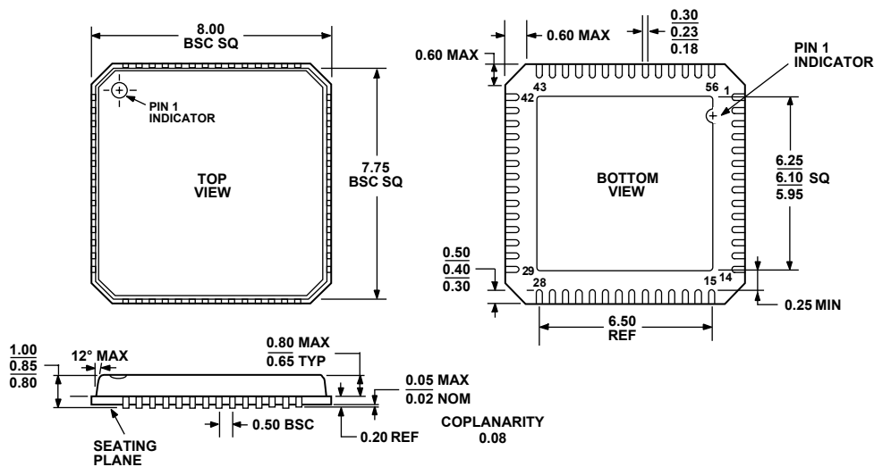
Figure 81. 56-Lead Frame Chip Scale Package [LFCSFP] (CP-56) Dimensions shown in millimeters
