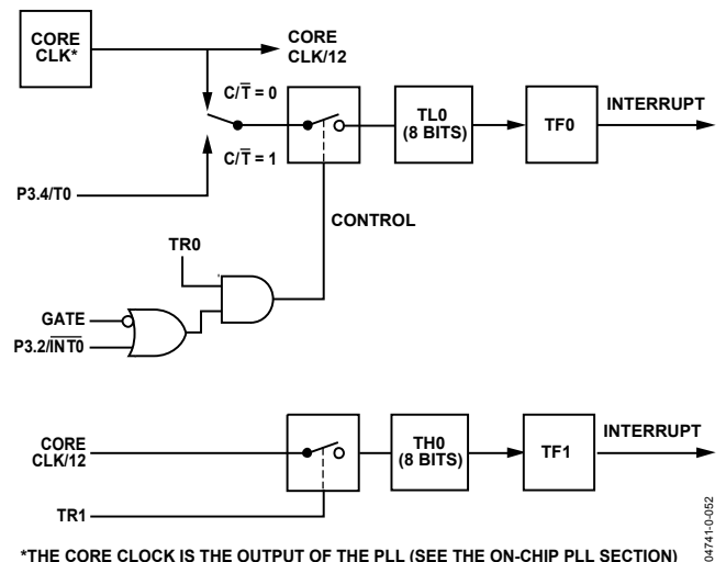
Figure 55. Timer/Counter 0, Mode 3
