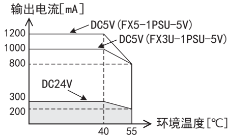
■FX5-1PSU-5V, FX3U-1PSU-5V的情况下
