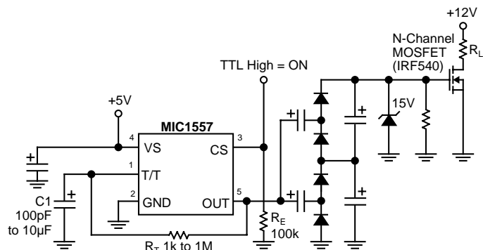
Figure 8. Charge-Pump
