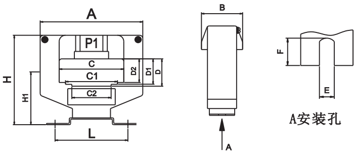
图4 LMZ3(D)-0.66 (750~3000) A
