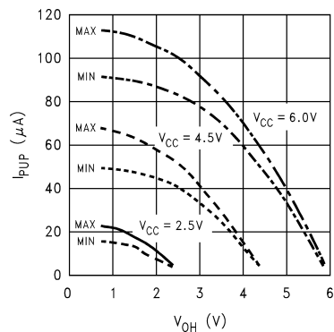
Port L/G Weak Pull-Up Source Current
