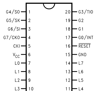
DUAL-IN-LINE PACKAGE 20 DIP
