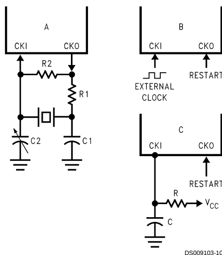
FIGURE 4. Crystal and R-C Connection Diagrams
