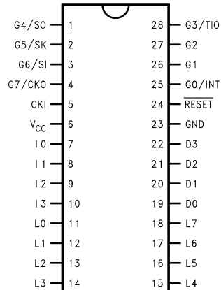
28-Lead SO
