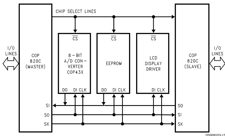
FIGURE 7. MICROWIRE/PLUS Application
