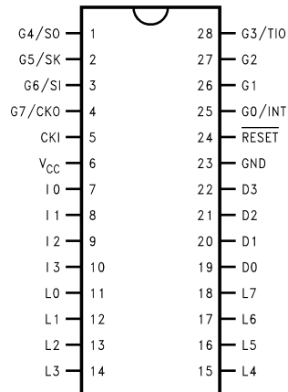
28 DIP
