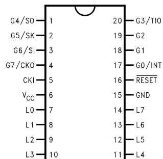
SURFACE MOUNT 20 SO Wide
