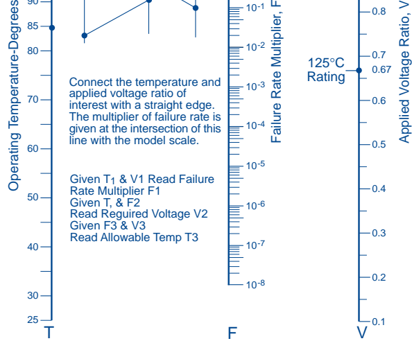
Figure 12. Reliability Nomograph
