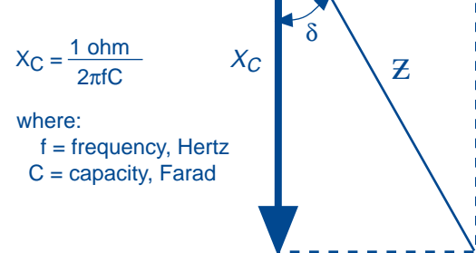
Figure 7a Total Impedance of the Capacitor Below Resonance
