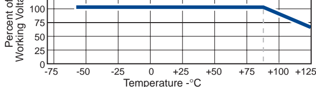
Figure 6. Working Voltage Change with Temperature
