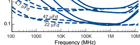
Figure 11a. ESR and Impedance vs. Frequency
