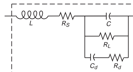
Figure 8. The Real Capacitor
