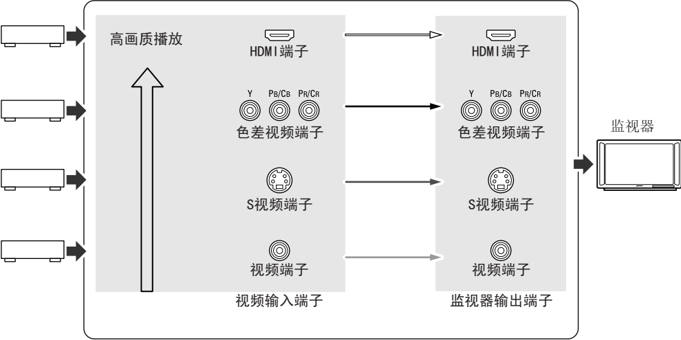
[AVR-1509内部视频信号的流向图]
