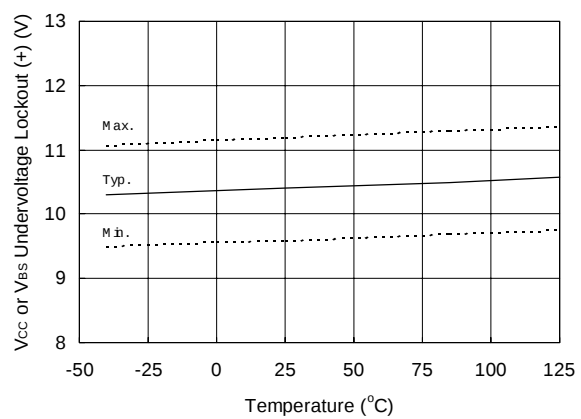
Figure 22. V_{CC} or V_{BS} Undervoltage Lockout (+) vs. Temperature (IR21362 Only)
