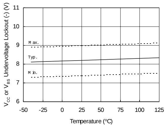
Figure 21. V_{CC} or V_{BS} Undervoltage Lockout (-) vs. Temperature (IR2136/IR21368 Only)
