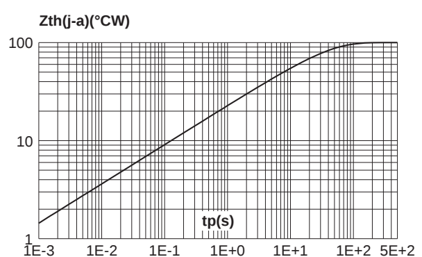
Fig. 6: Variation of thermal impedance junction to ambient versus pulse duration (Printed circuit board FR4, SCu=35μm, recommended pad layout).
