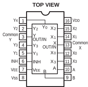
BU4052BCF (AU:IC255,509,510)
