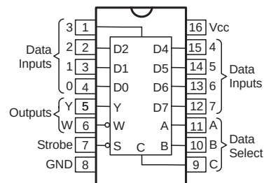
SN74HC151NS (EX:IC505,506)
