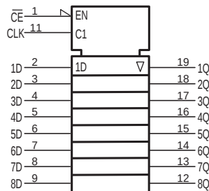
logic symbol
