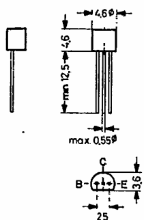
TO-92 Plastic Package Pins in-Line "D" Weight approx. 0.18 g
