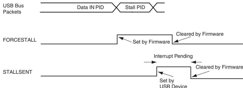
Figure 39-13. Stall Handshake (Data IN Transfer)
