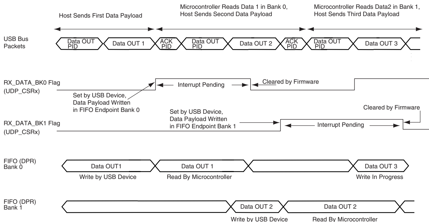
Figure 39-12. Data OUT Transfer for Ping-pong Endpoint
