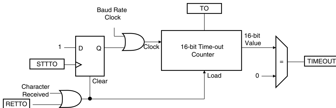
Figure 34-14. Receiver Time-out Block Diagram
