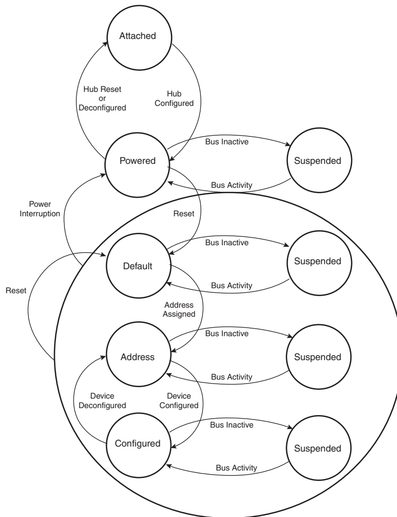
Figure 39-15. USB Device State Diagram
