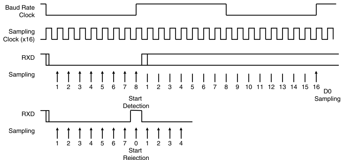
Figure 34-8. Asynchronous Start Detection
