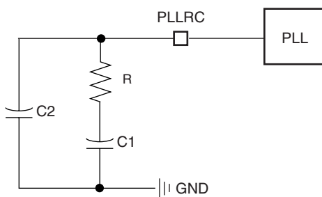
Figure 27-5. PLL Capacitors and Resistors
