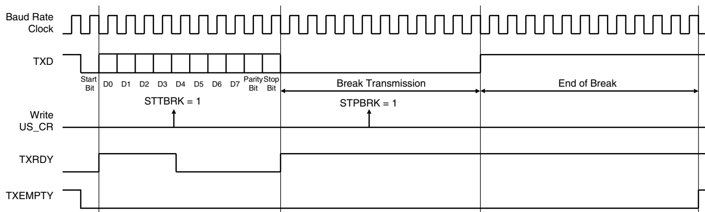
Figure 34-16. Break Transmission
