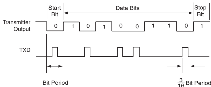
Figure 34-24. IrDA Modulation
