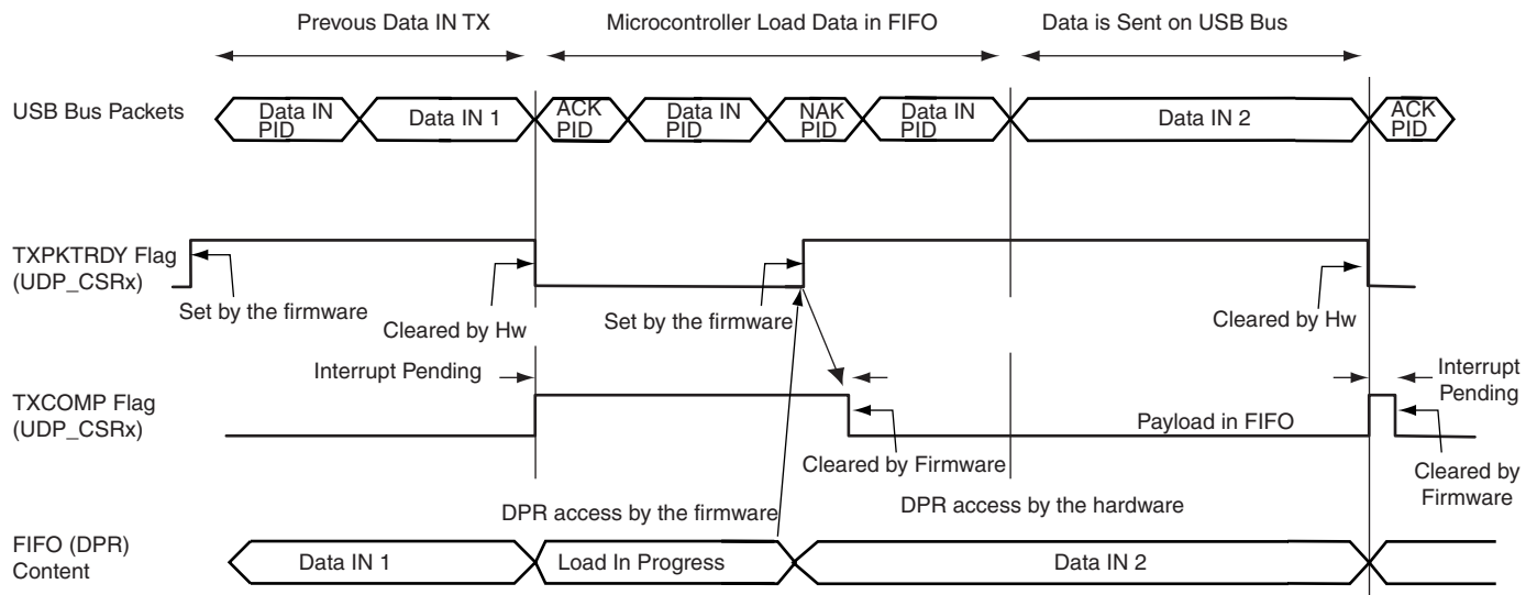
Figure 39-7. Data IN Transfer for Non Ping-pong Endpoint
