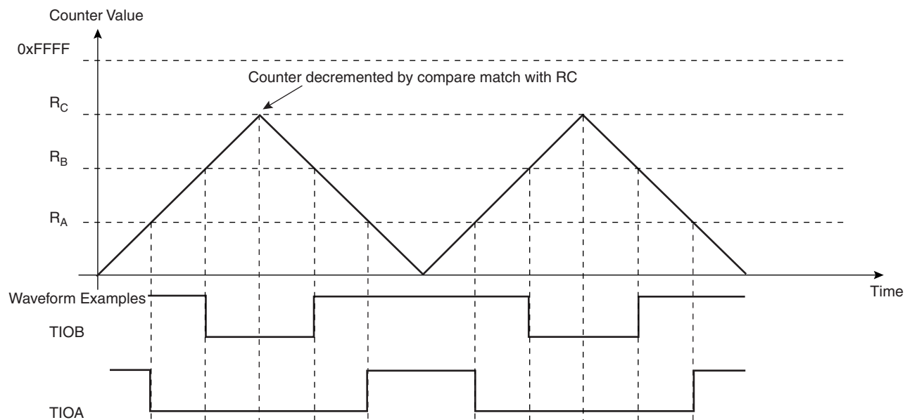
Figure 39-13. WAVSEL = 11 Without Trigger
