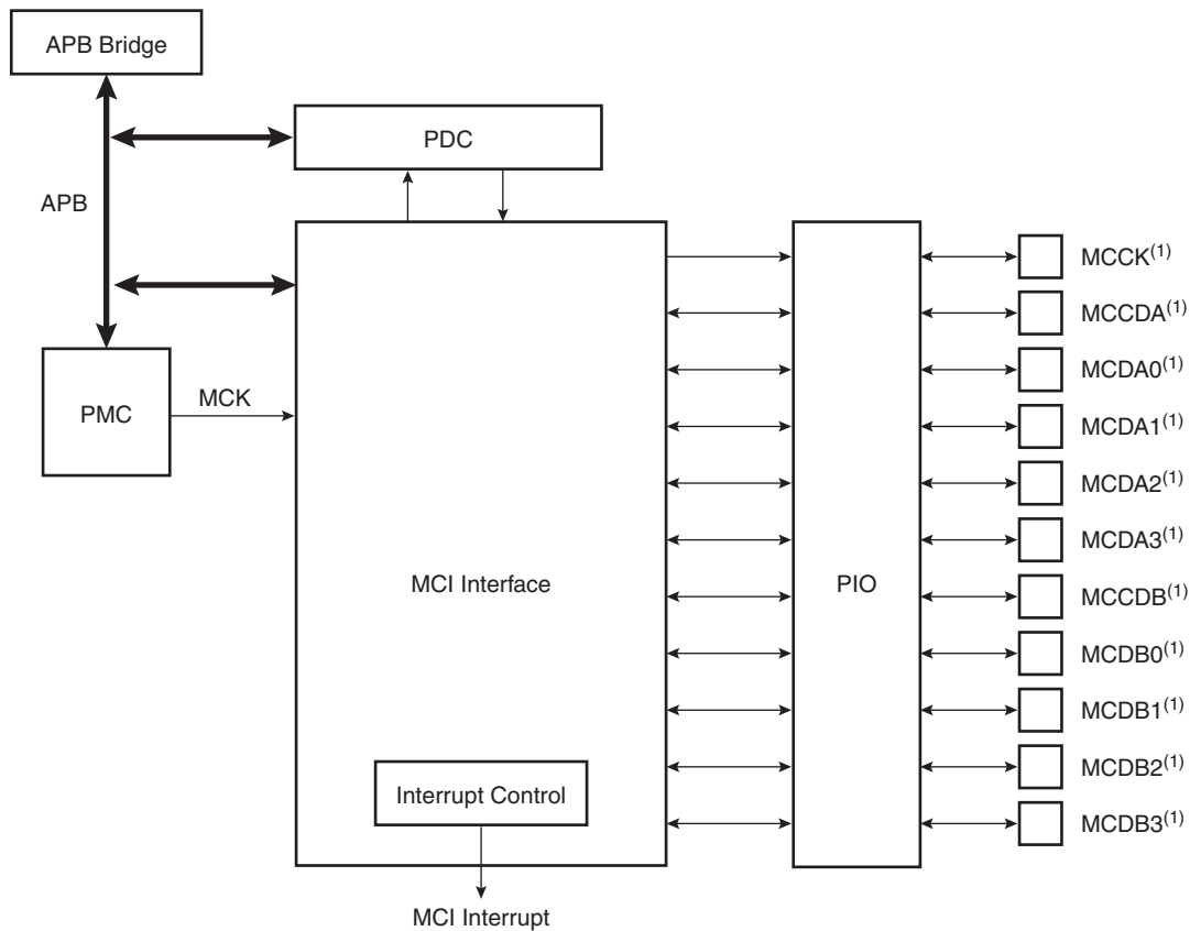
Figure 40-1. Block Diagram
