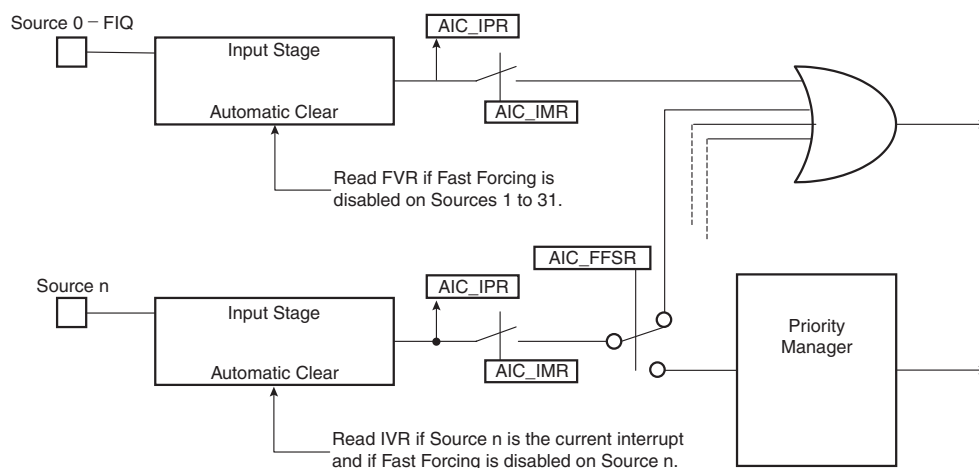
Figure 29-10. Fast Forcing
