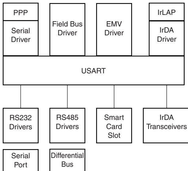
Figure 34-2. Applicatio Block Diagram
