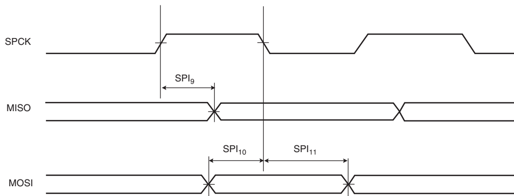
Figure 47-11. SPI Slave Mode with (CPOL = NCPHA = 0) or (CPOL= NCPHA= 1)
