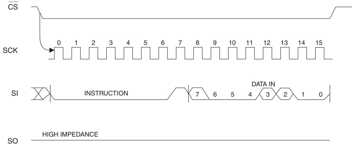
Figure 4-5. WRSR Timing
