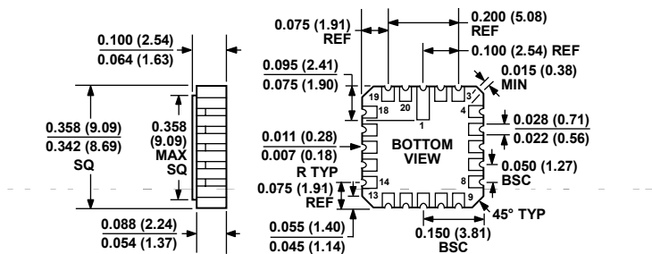
Figure 59. 20-Terminal Ceramic Leadless Chip Carrier [LCC] (E-20-1) RC-Suffix
