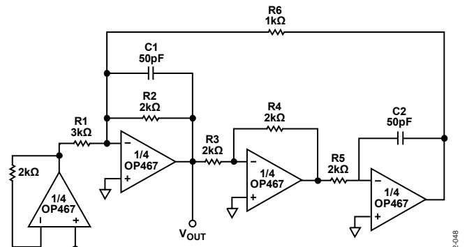
Figure 48. 2 MHz Biquad Filter
