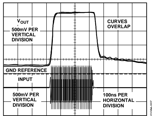
Figure 13. Large-Signal RSSI Pulse Response with R_L = 100 \Omega and C_L = 33 pF, 68 pF, and 100 pF
