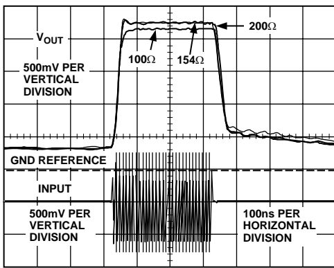
Figure 10. Large-Signal RSSI Pulse Response with C_L = 100 pF and R_L = 100 \Omega , 154 \Omega , and 200 \Omega
