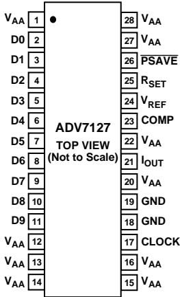
28-Lead SOIC
