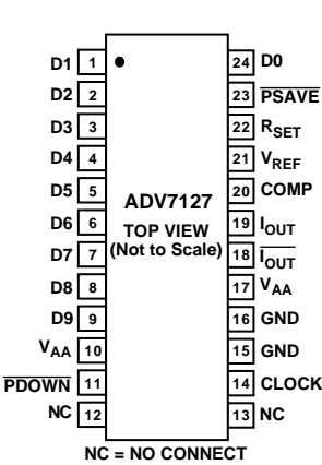
24-Lead TSSOP
