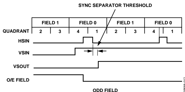
Figure 12. VSYNC Filter—Odd
