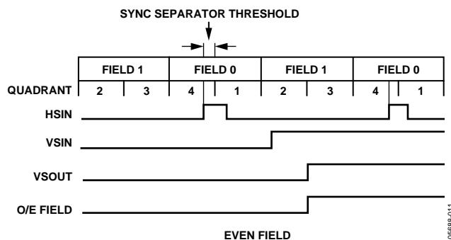
Figure 11. VSYNC Filter—Even
