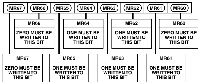
Figure 29. Mode Register 6
