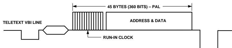
Figure 72. Teletext VBI Line
