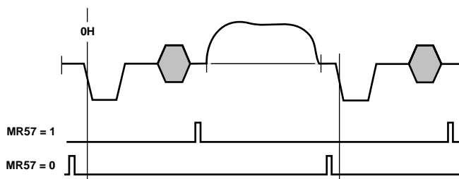
Figure 38. Clamp Output Timing
