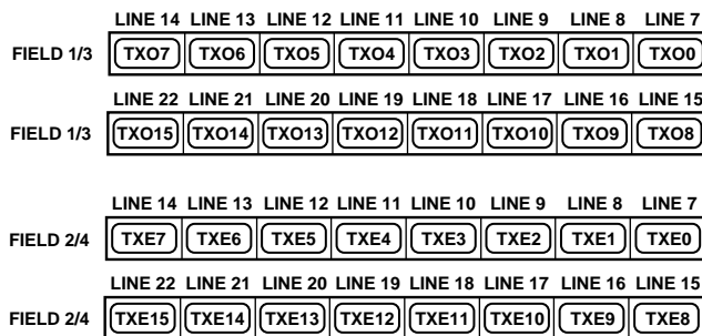
Figure 58. Teletext Control Registers
