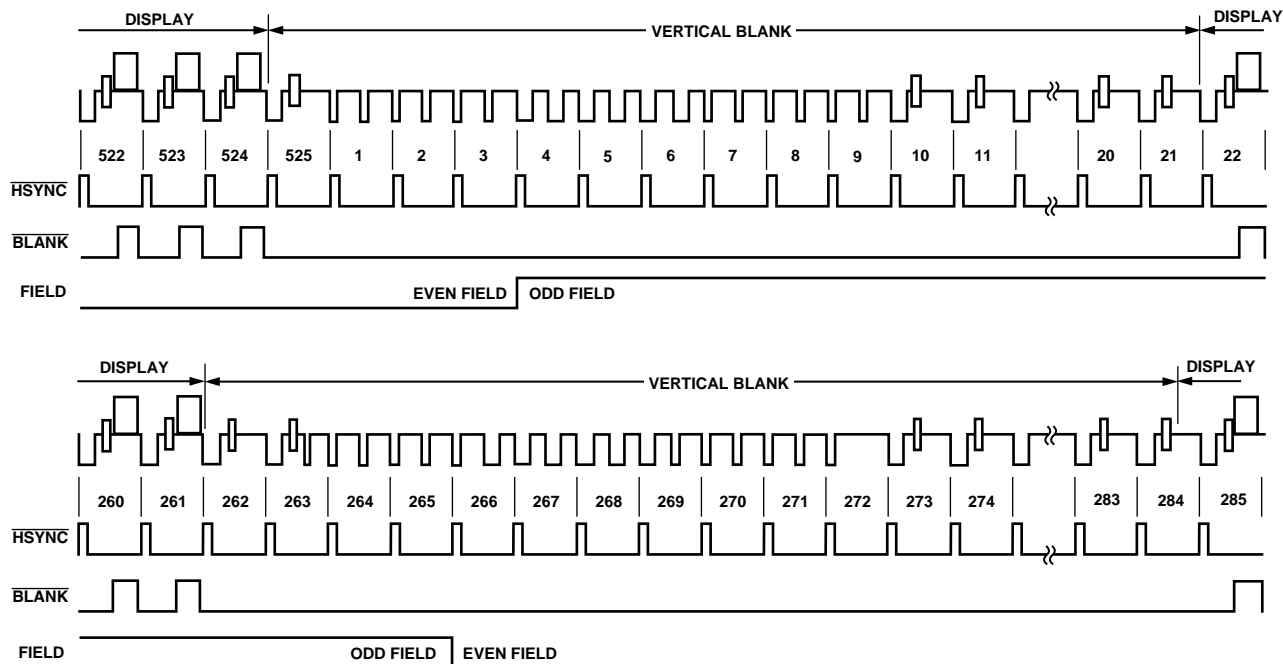
Figure 34. Timing Mode 3 (NTSC)
