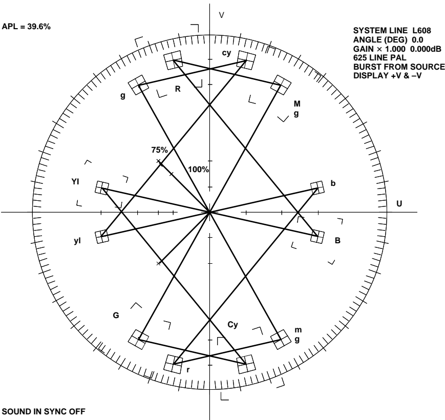
Figure 102. PAL Vector Plot
