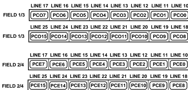
Figure 57. Pedestal Control Registers
