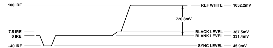
Figure 64. NTSC RGB Video Levels
