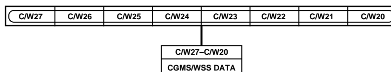
Figure 52. CGMS_WSS Register 1
