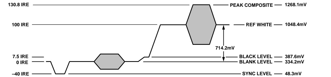
Figure 61. NTSC Composite Video Levels
