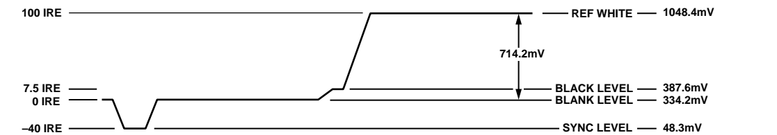
Figure 62. NTSC Luma Video Levels
