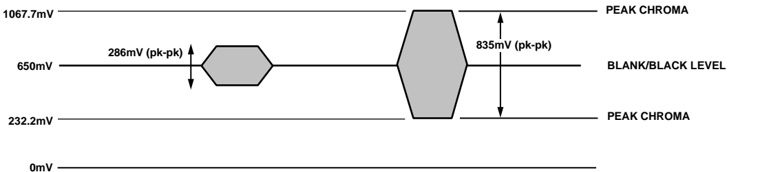
Figure 63. NTSC Chroma Video Levels
