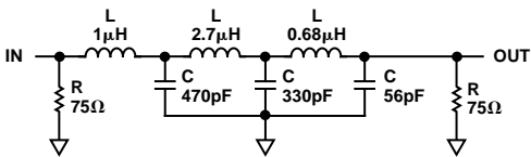
Figure 79. Output Filter
