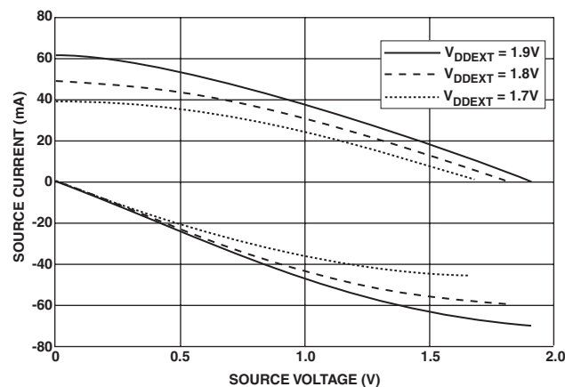
Figure 32. Drive Current B ( V_{DDEXT} = 1.8 \text{ V} )
