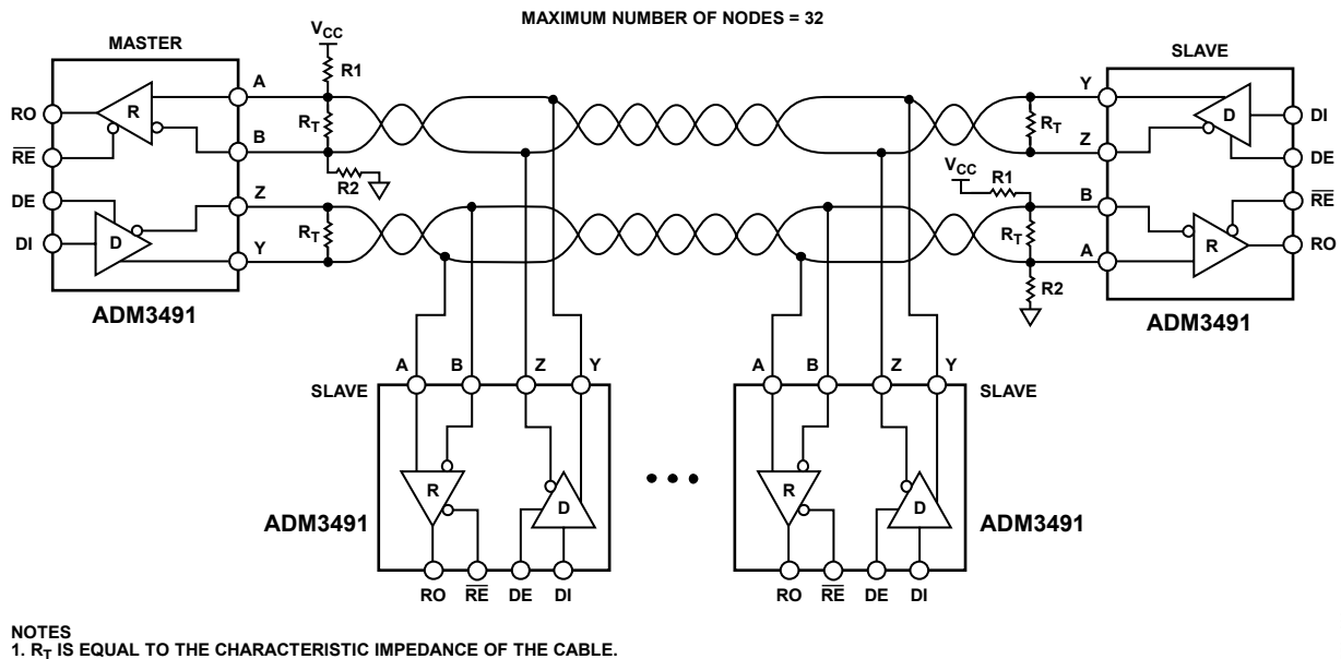
Figure 33. ADM3491 Typical Full-Duplex RS-485 Network
