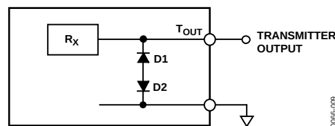
Figure 9. Transmitter Output Protection Scheme
