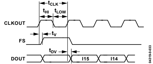
Figure 33. SSI Timing Parameters for SSI Timing*
