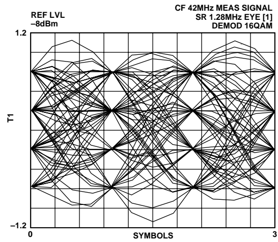
Figure 18. 16-QAM Modulation
