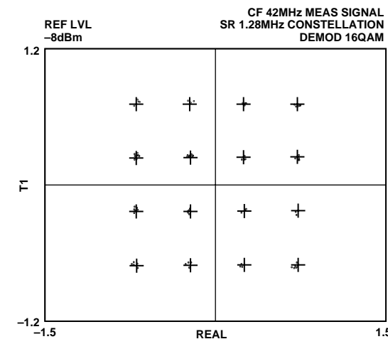
Figure 19. 16-QAM Modulation
