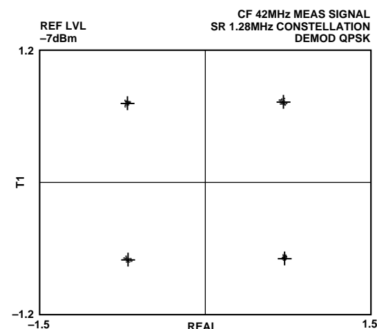
Figure 17. QPSK Modulation
