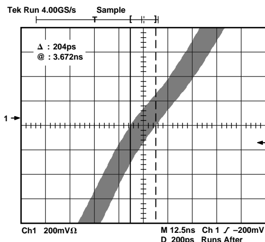
Figure 33. Typical CMOS comparator p-p output jitter with the AD9851 configured as a clock generator, \text{DDS } f_{\text{OUT}} = 40.1 MHz, V_S = +5 V, system clock = 180 MHz, 70 MHz LPF. Graph details the center portion of a rising edge with scope in delayed trigger mode, 200 ps/div. Cursors show 204 ps p-p jitter.
