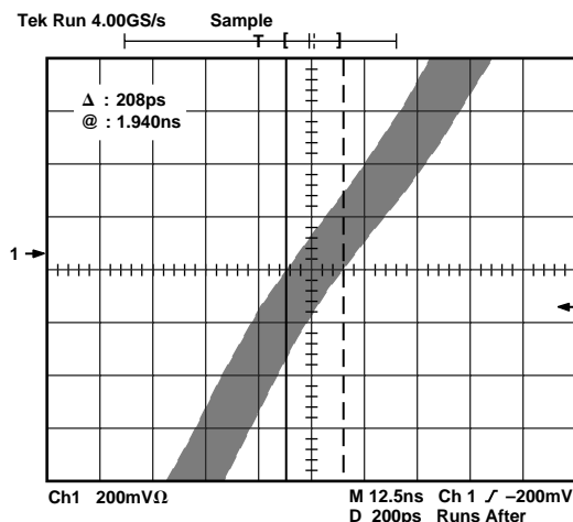
Figure 32. Typical CMOS comparator p-p output jitter with the AD9851 configured as a clock generator, \text{DDS } f_{\text{OUT}} = 10.1 MHz, V_S = +5 V, system clock = 180 MHz, 70 MHz LPF. Graph details the center portion of a rising edge with scope in delayed trigger mode, 200 ps/div. Cursors show 208 ps p-p jitter.
