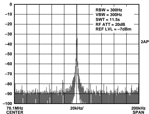
Figure 31. Narrowband ( 70.1 \pm 0.1 MHz) output SFDR for a 70.1 MHz fundamental output signal. System clock = 180 MHz ( 6 \times \text{REFCLK Multiplier} engaged), V_S = +5 V.
