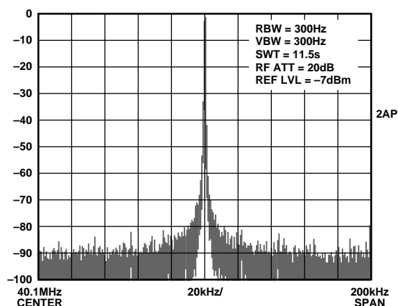
Figure 30. Narrowband ( 40.1 \pm 0.1 MHz) output SFDR for a 40.1 MHz fundamental output signal. System clock = 180 MHz ( 6 \times \text{REFCLK Multiplier} engaged), V_S = +5 V.
