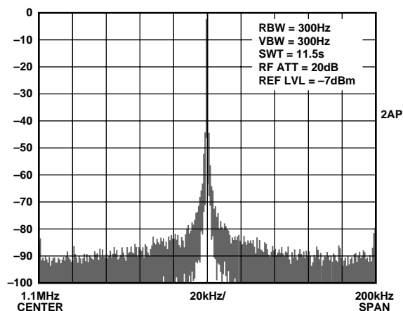
Figure 29. Narrowband ( 1.1 \pm 0.1 MHz) output SFDR for a 1.1 MHz fundamental output signal. System clock = 180 MHz ( 6 \times \text{REFCLK Multiplier} engaged), V_S = +5 V.
