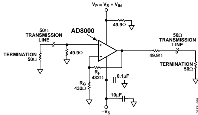
Figure 48. Positive PSRR
