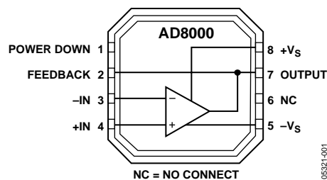
Figure 1. 8-Lead AD8000, 3 mm \times 3 mm LFCSP (CP-8-2)
