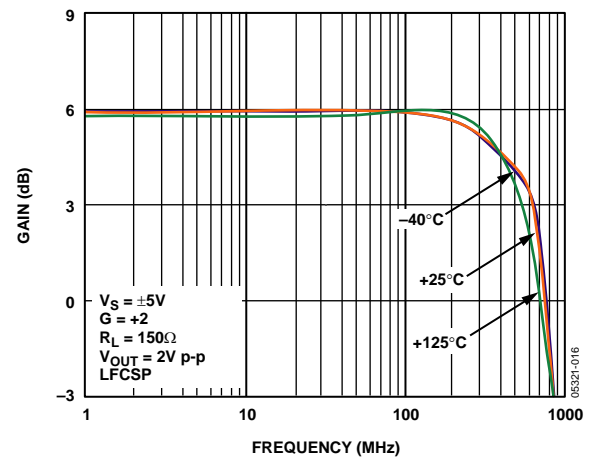
Figure 16. Large Signal Frequency Response vs. Temperature
