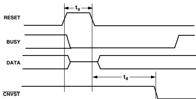
Figure 12. RESET Timing
