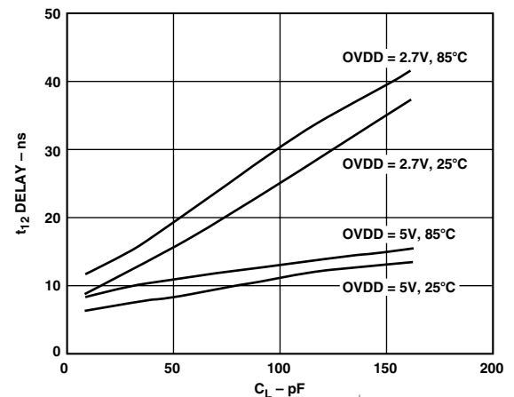
TPC 12. Typical Delay vs. Load Capacitance C_L
