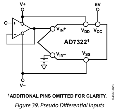
Figure 39. Pseudo Differential Inputs
