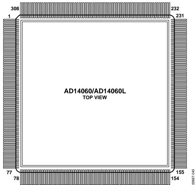
Figure 20. 308-Lead CQFP Pin Configuration
