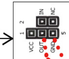
B. JSPDIF Pin Assignment
