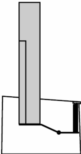
Patent design for HDD depart from docking unit
